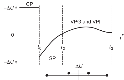
Fig. 11. Schematic of the transient over the conducting polarizing medium in the equatorial region of the source for the symmetric array. t_0 , current turn-off time; t_2 , the time at which the field sign changes with the manifestation of IP (VPG and VPI); t_3 , end of measurements. See the remaining denotations in Fig. 10.
