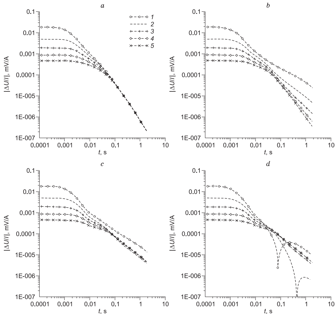
Fig. 4. Absolute values of the transient signal on the measuring lines with a separation of 1500 (1), 2500 (2), 3500 (3), 4500 (4), and 5500 (5) m: a , above the nonpolarized medium; b , above the medium polarized in the upper part of the section; c , above the polarized medium; d , above the medium polarized over the high-resistance screen.
