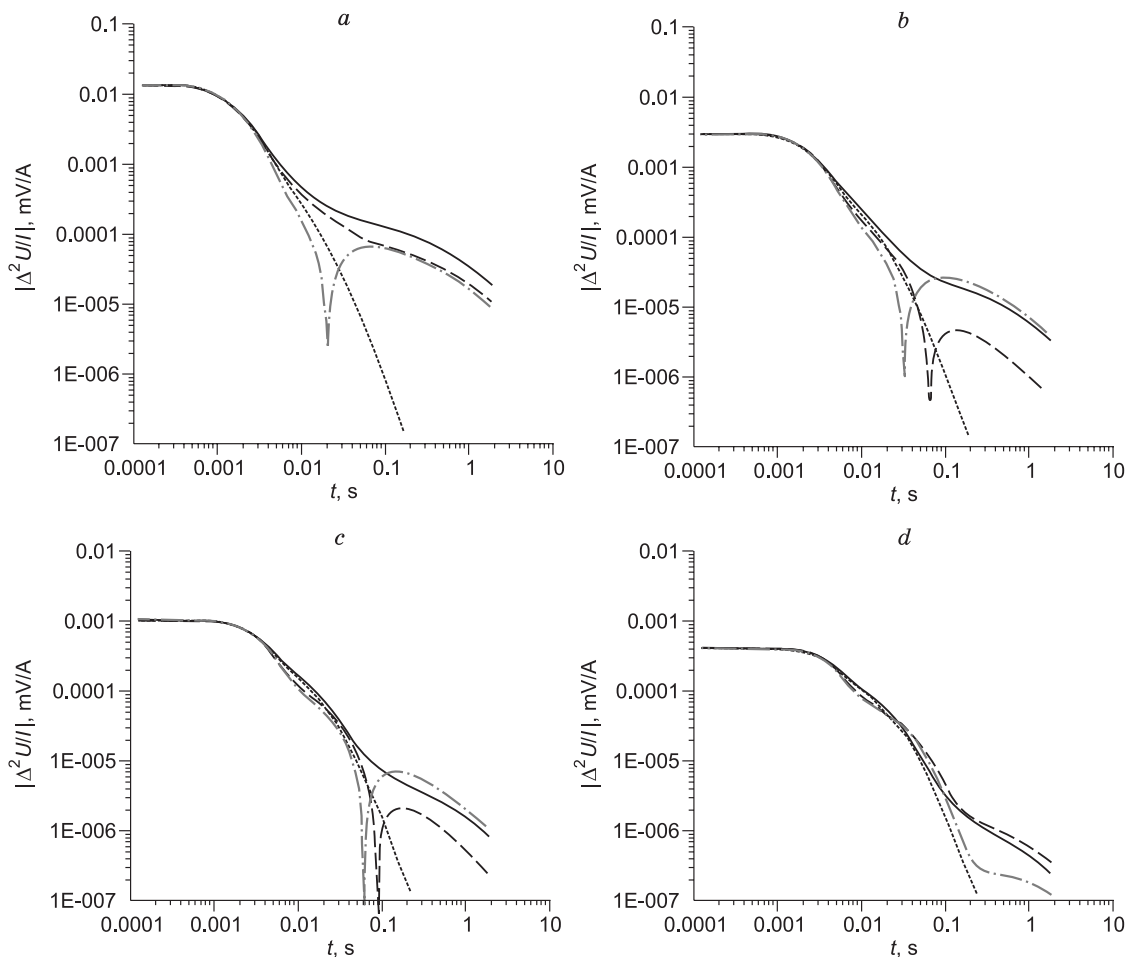
Fig. 8. Absolute values of the transient response of the second final potential difference on the 3-electrode measuring lines M_1M_2M_3 (a), M_2M_3M_4 (b), M_3M_4M_5 (c), and M_4M_5M_6 (d). See denotations in Fig. 6.
