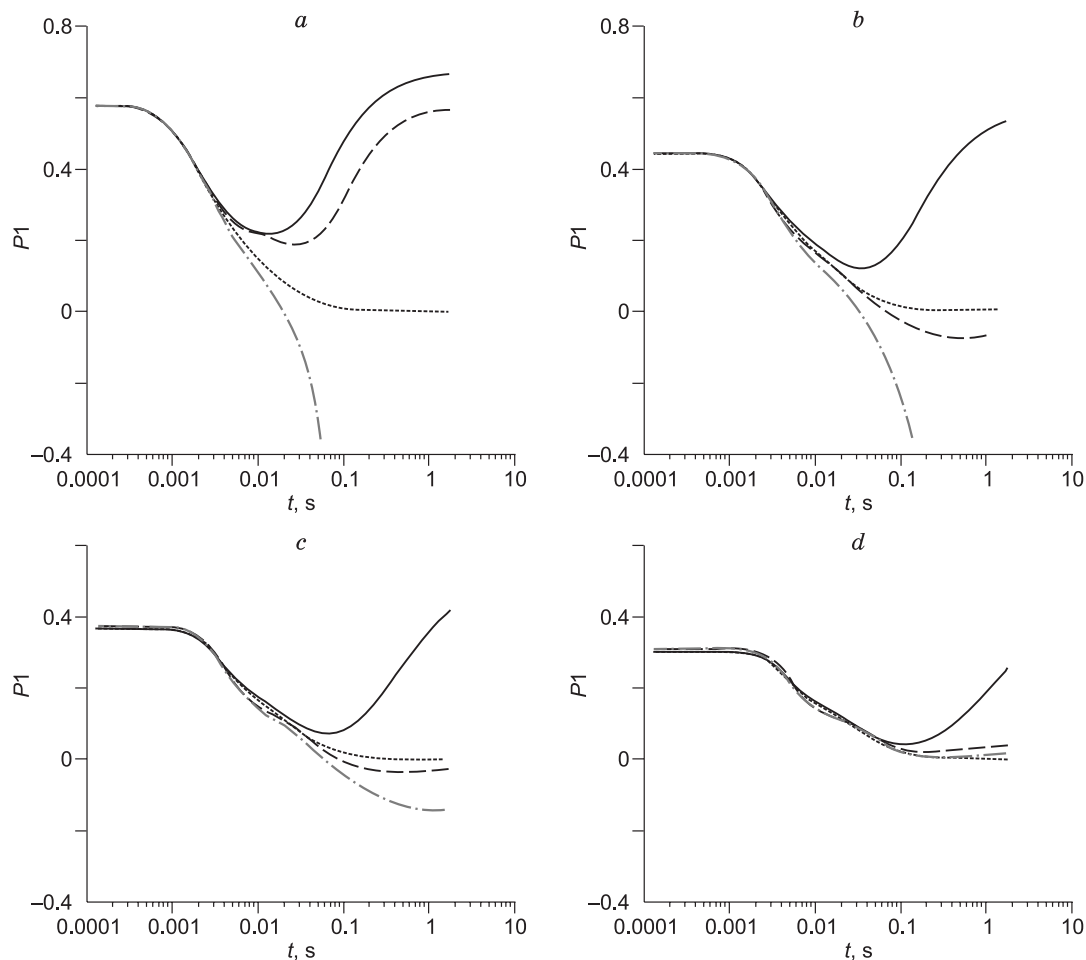
Fig. 9. Transient response of transform P1 on the 3- electrode measuring lines M_1M_2M_3(a) , M_2M_3M_4(b) , M_3M_4M_5(c) , and M_4M_5M_6(d) . See denotations in Fig. 6.
