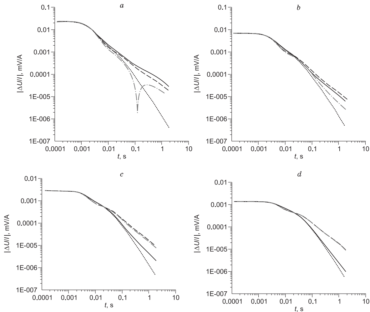
Fig. 7. Absolute values of the transient signal on the 3-electrode measuring lines M_1M_2M_3 (a), M_2M_3M_4 (b), M_3M_4M_5 (c), and M_4M_5M_6 (d). See denotations in Fig. 6.
