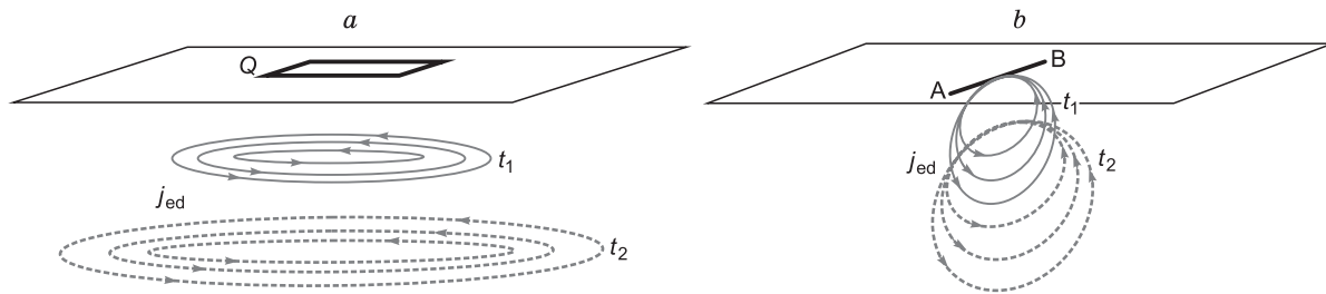
Fig. 1. Simplified structure of eddy currents: a , for the inductive loop source ( Q ); b , for the grounded line source ( AB ). j_{ed} , main eddy current density; t_1 and t_2 , instances for which the eddy current density is shown.
