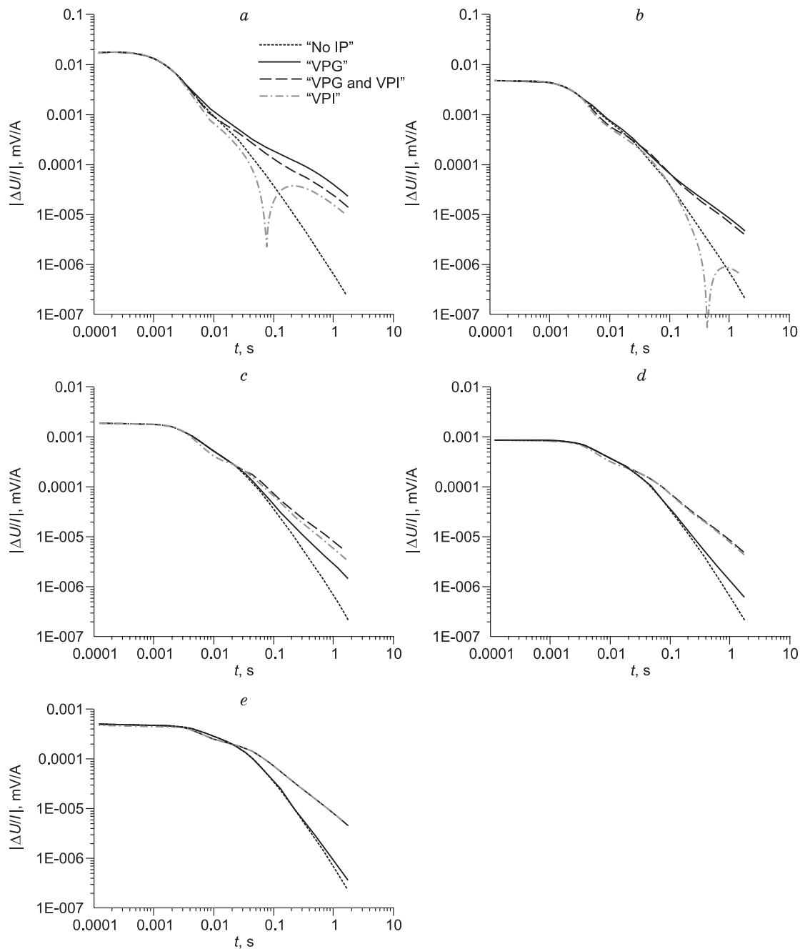
Fig. 6. Absolute values of the transient signal from four models on the measuring lines located at a distance of: a , 1500; b , 2500; c , 3500; d , 4500; e , 5500 m.
