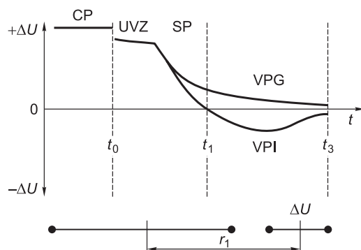
Fig. 10. Schematic of the transient over the conducting polarizing medium in the axial region of the source at small separations. CP, current pulse; UVZ, pulse excitation propagating through the air; SP, process of EM field formation; VPG, galvanic induced polarization; VPI, inductive induced polarization; t_0 , the current turn-off time; t_1 , the time at which the field sign changes with the manifestation of IIP; t_3 , end of measurements, r_1 , separation close to the size of the source.
