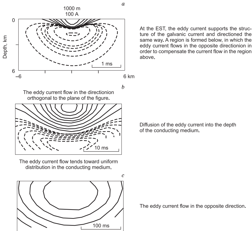
Fig. 2. Isolines of the eddy current density at different times of the transient, according to Strack (1992).
