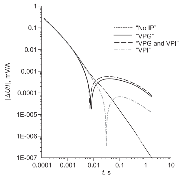
Fig. 5. Absolute values of the transient signal from four models on the symmetrical measuring line.
