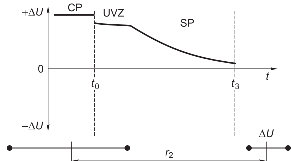
Fig. 12. Schematic of the transient over the conducting polarizing medium in the axial region of the source at large separations. See denotations in Fig. 10. r_2 , separation several times larger than the size of the source.
