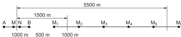
Fig. 3. Array for the numerical experiment. Measuring lines in the axial ( M_1M_2 , M_2M_3 , M_3M_4 , M_4M_5 , M_5M_6 ) and equatorial (MN) regions of the source (AB).
